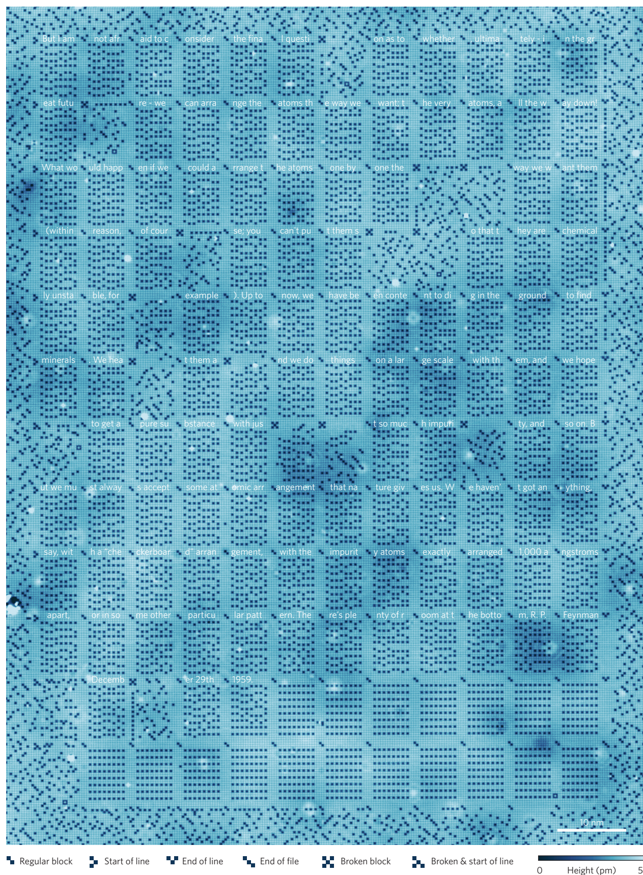
Figure 3 | Kibibyte atomic memory. STM image ( 96 \times 126 nm, I = 2.00 nA, V = +500 mV, T = 1.5 K) of a 1,016-byte atomic memory, written to a passage from Feynman's lecture 'There's plenty of room at the bottom' 26 . The various markers used are explained in the legend below the images. The memory consists of 127 functional blocks and 17 broken blocks, resulting in an overall areal density of 0.778 bits nm -2 .
