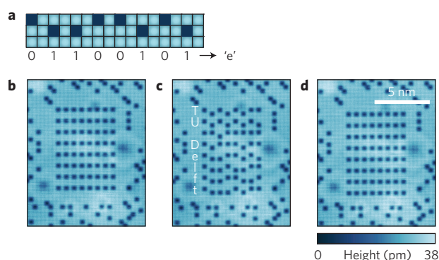
Figure 2 | Data-encoding principle. a , Diagram showing the smallest possible byte, provided that vacancies are not direct neighbours. The byte is set to represent the binary ASCII code for the character 'e'. b–d , STM images ( I = 2.00 nA, V = +500 mV, T = 1.5 K) of a 64-bit block, written as all 0s ( b ), a text ( c ) and all 1s ( d ).
