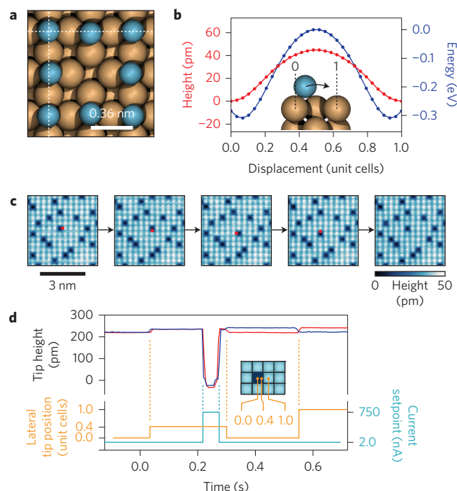
Figure 1 | Hopping mechanism of a Cl vacancy on chlorinated Cu(100).
